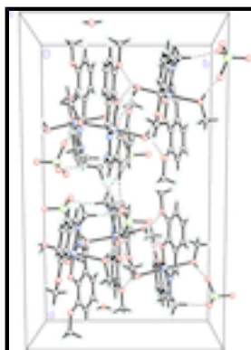
Fig. 2. The molecular packing for C 38 H 50 Cl 2 Mn 2 N 4 O 21 viewed down the c axis. Hydrogen bonds are shown by dashed lines.
